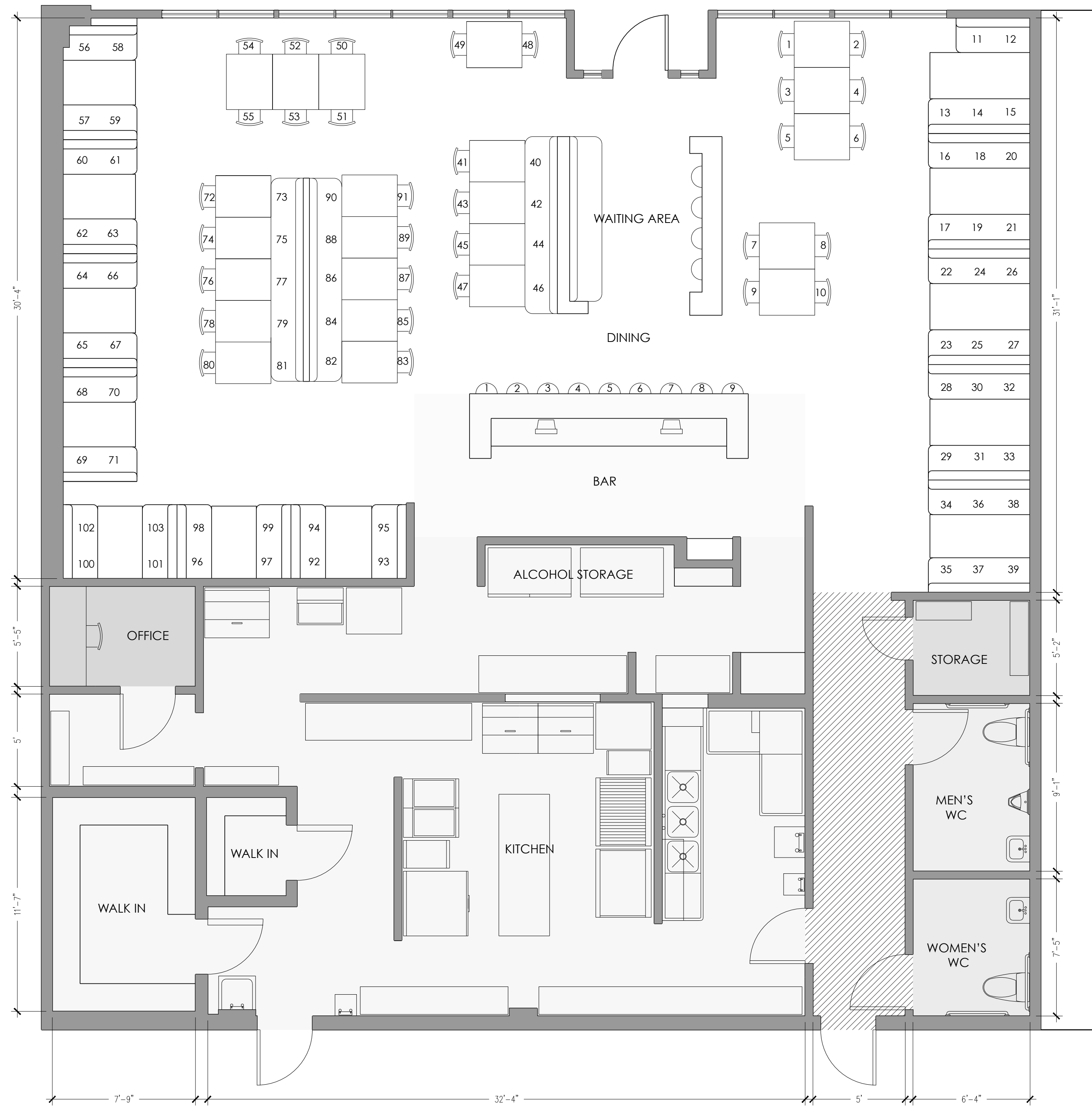
1 RESTAURANT FLOOR PLAN SCALE 1/4" = 1'-0"
